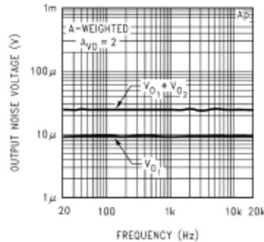
Noise Floor
